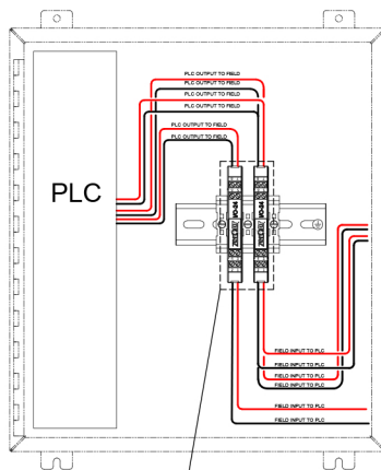
CONTROL CABINET
